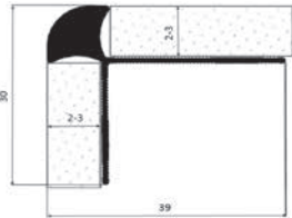
STAIR PROFILE STEEL, DRY BACK
