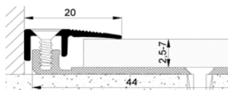
END MOULDING STEEL
