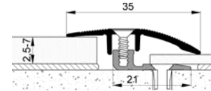
BEVEL COVER STRIP STEEL
