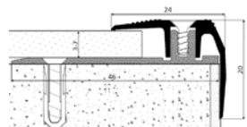
STAIR NOSE STEEL
